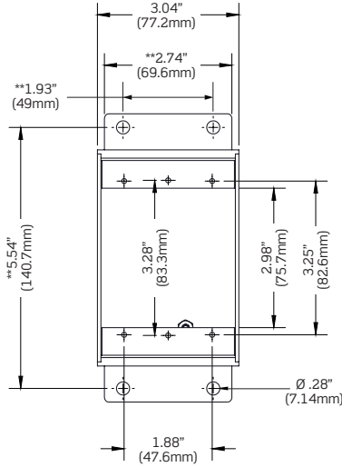
Single-Gang Front View
