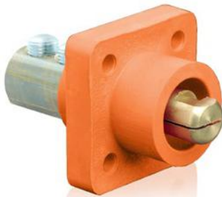
Male Panel Mount Receptacle - Double Set Screw (18R23-UO Shown)
